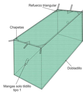
Figura 1. Vista general toldillo
